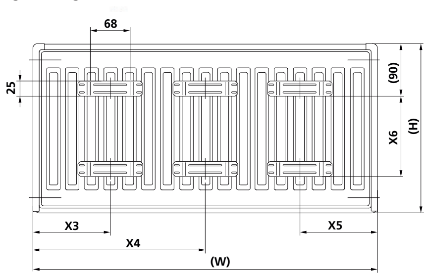
Fig 1 - Fixing Positions for Brackets
