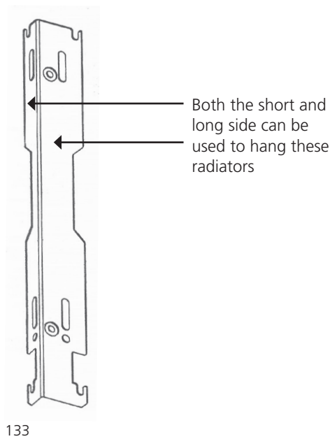
Bracket drawing
